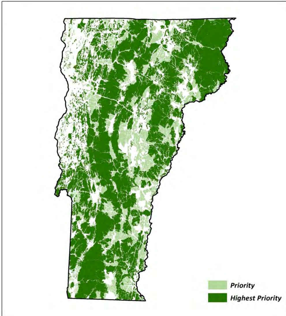
Map 1. The Highest Priority and Priority portions of the Ecologically Functional Landscape, including Interior Forest Blocks, Connectivity Blocks, and Physical Landscape Diversity Blocks (excluding the Surface Waters and Riparian Areas which are difficult to interpret at this scale).
